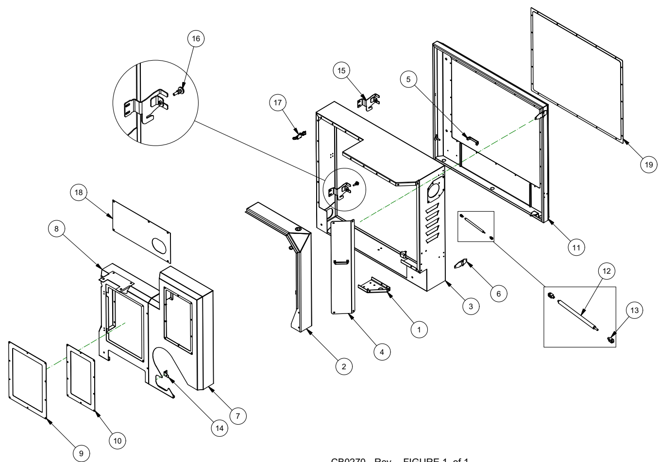
CB0270 - Rev- - FIGURE 1 of 1
