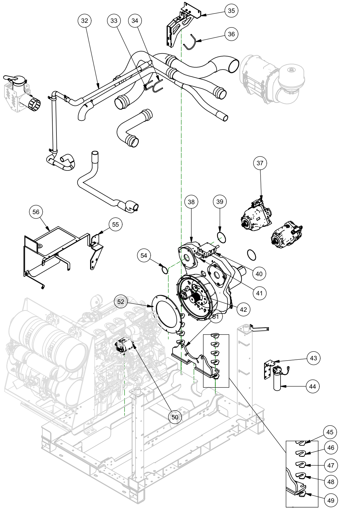
CB0264 - RevD - FIGURE 3 of 3
