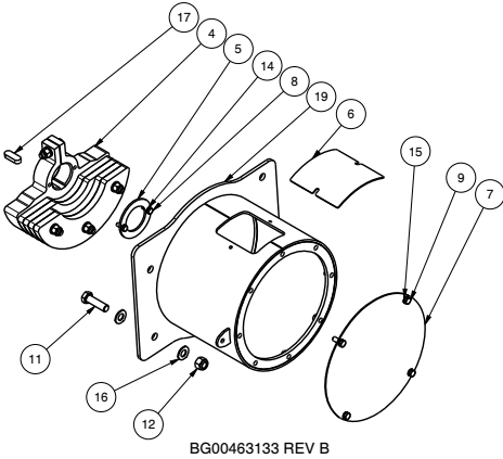
BG00463133 REV B
