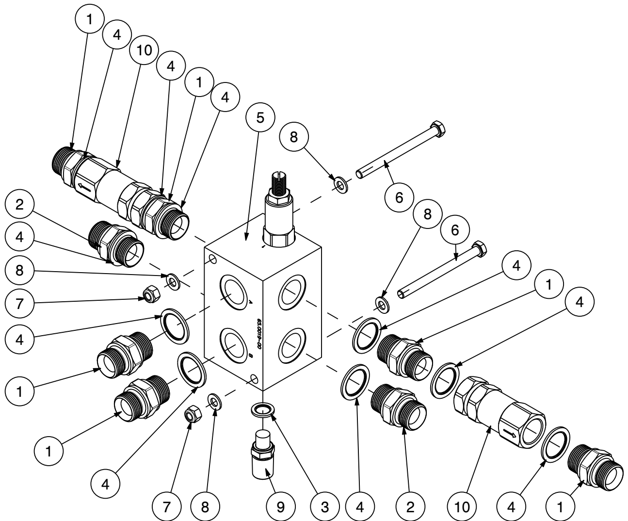
BG00500104 REV A
