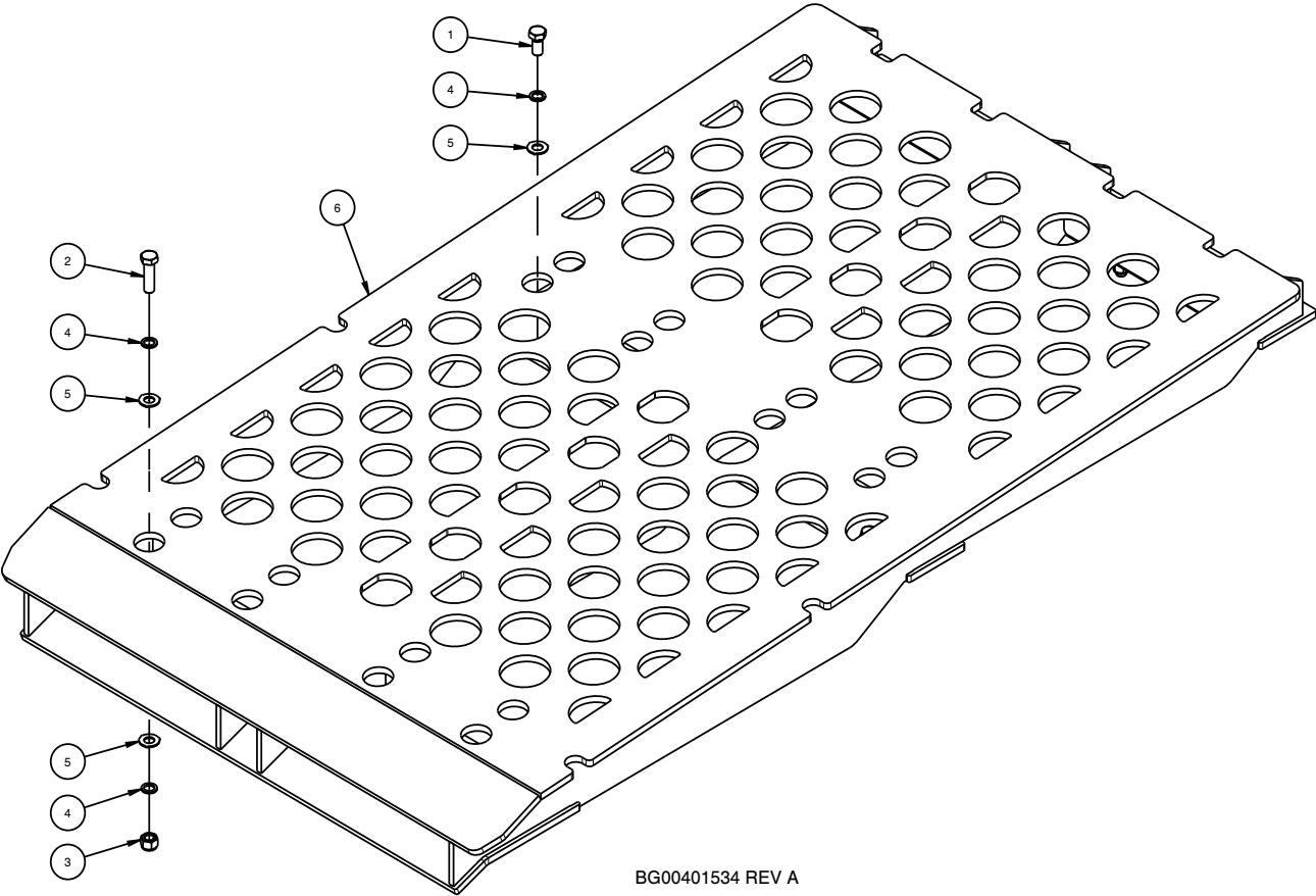
BG00401534 REV A
